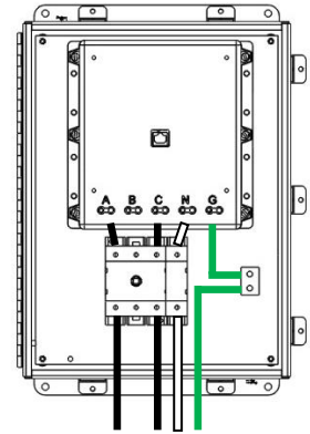
3-Phase WYE, 4-Wire + Ground D200M-120/2083YT, D300M-120/2083YT D200M-277/4803YT, D300M-277/4803YT
